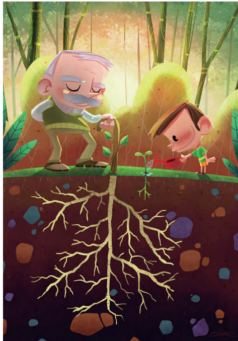
Root
