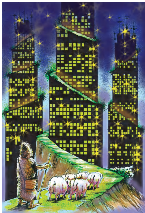
City
